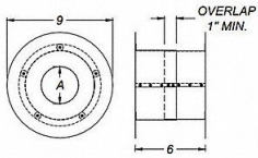
Horizontal Wall Thimble - Round Face
